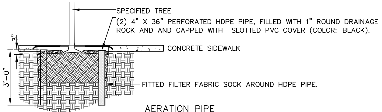
AERATION PIPE
